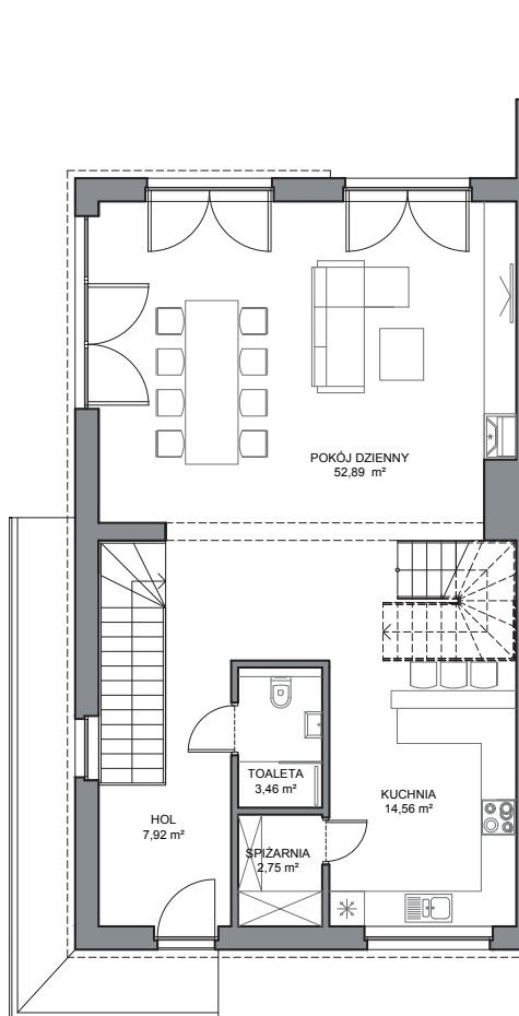
PARTER 81,58 m 2
